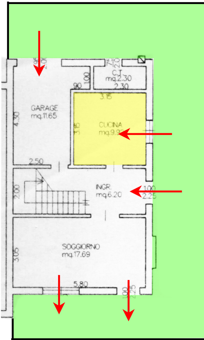
PIANO TERRA
